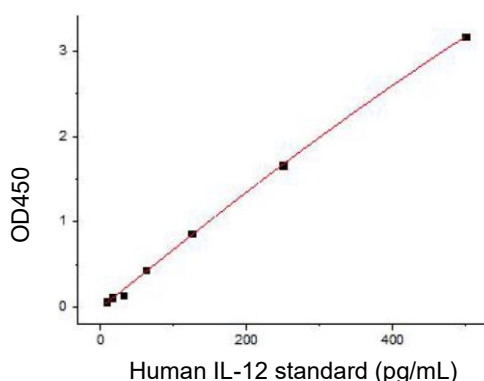
Figure1. Standard Curve of Human IL-12 in 96-well plate assay, data provided for demonstration purposes only. A new standard
